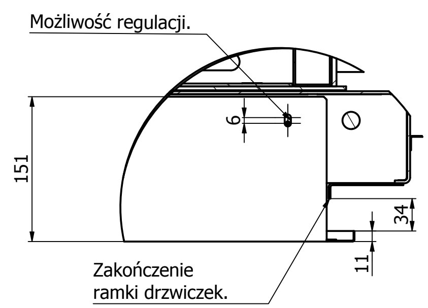
C (1:4)
