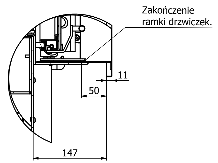
C (1:4)
