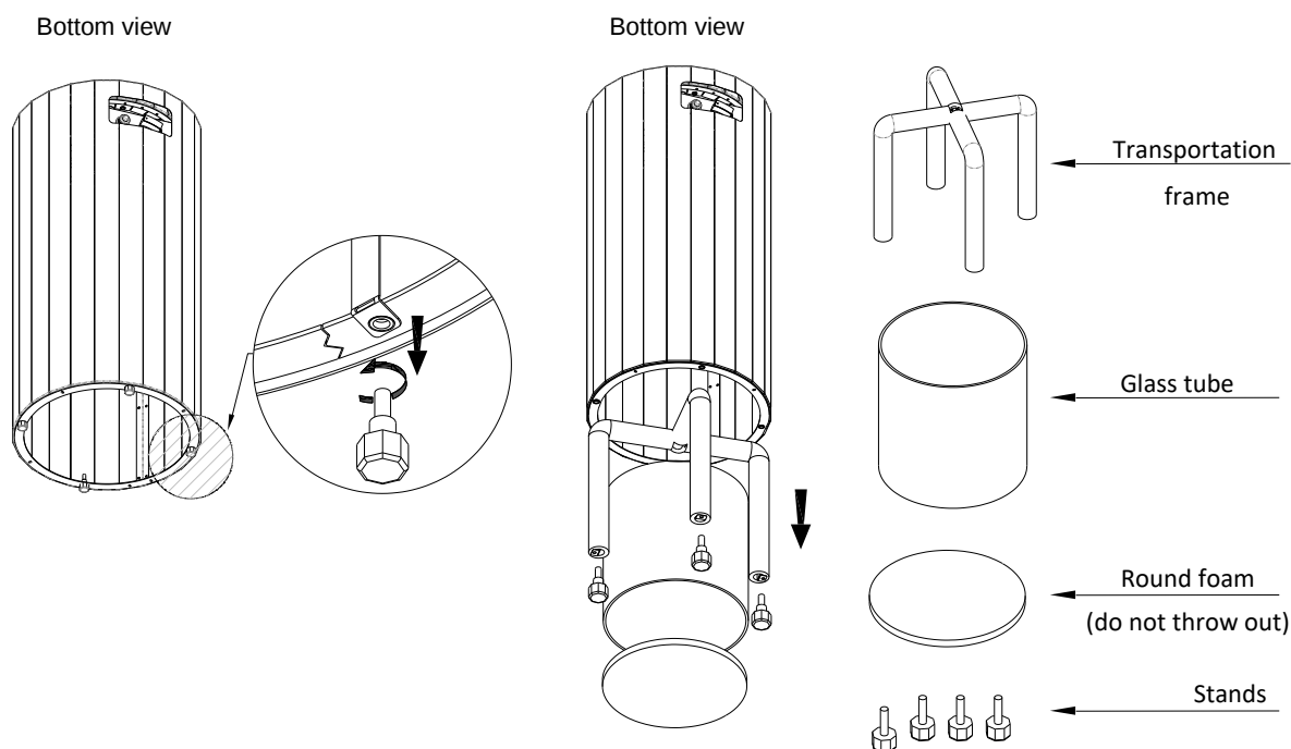
Fig. 2 – Unassembling transportation frame
