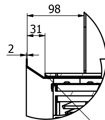
A (1:4)
