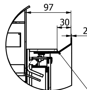
C (1:4)
