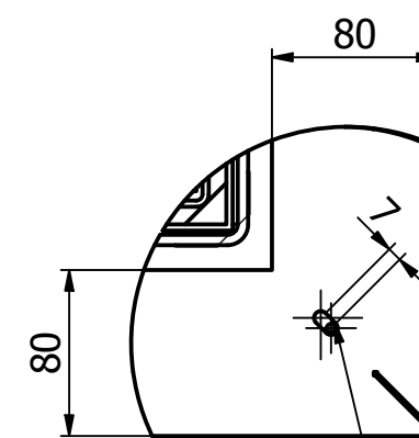
E (1:4)
