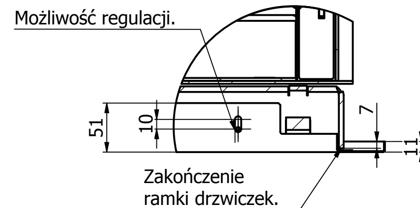
C (1:4)
