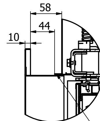
A (1:4)
