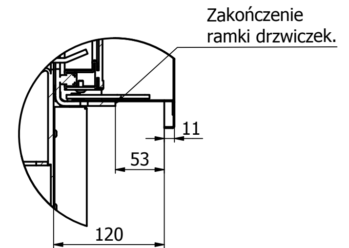
B (1:4)
