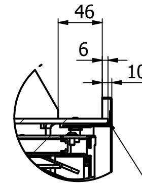
C (1:4)
