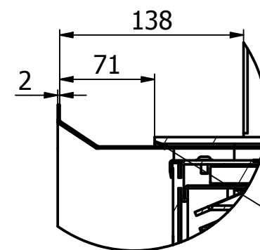
A (1:4)
