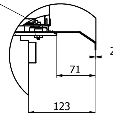
D (1:4)
