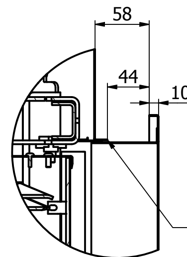
C (1:4)
