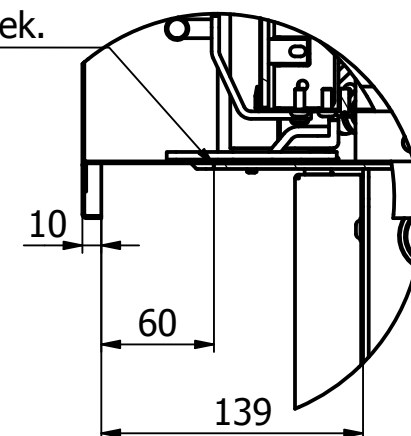
D (1:4)
