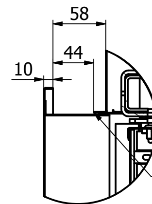
A (1:4)
