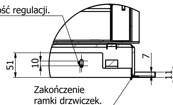
C (1:4)
